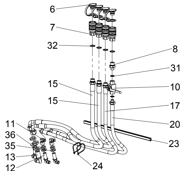
Rapid AC 2000/2500/3000
