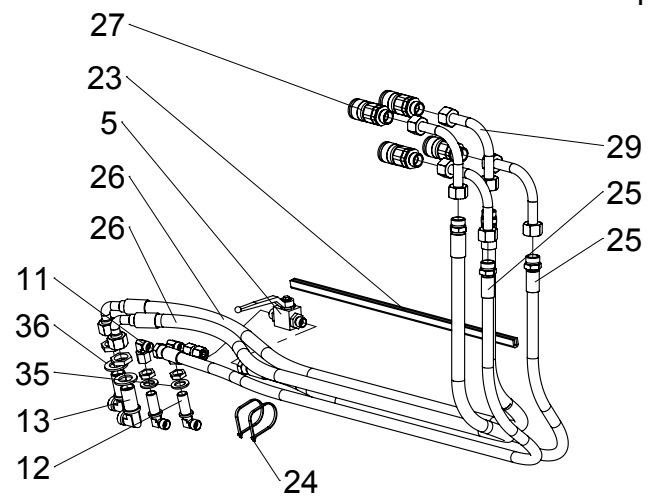
Lindner Unitrac 82/92/102
