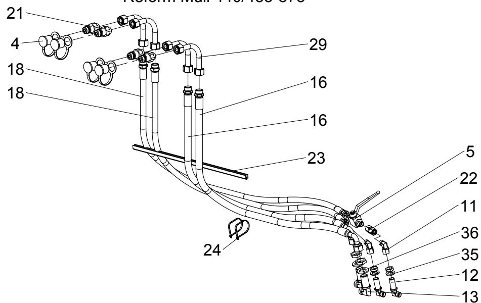
Reform Muli 440/455-875
