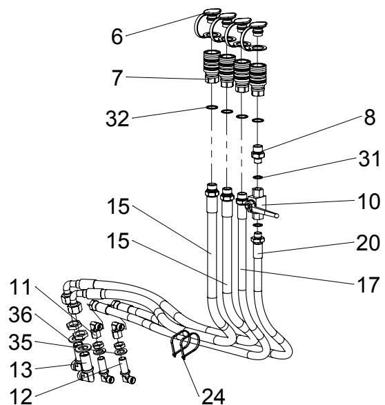
Lindner Unitrac 95
