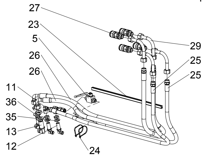
Lindner Unitrac 82/92/102
